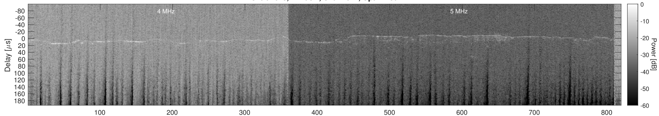
Orbit 4618, Cluttergram
