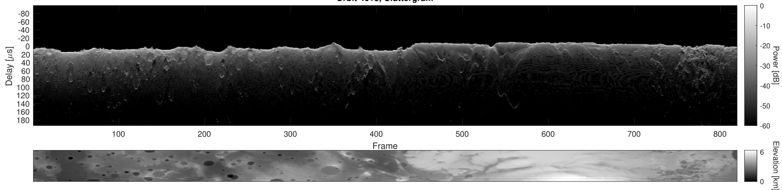
Orbit 4618, Cluttergram
