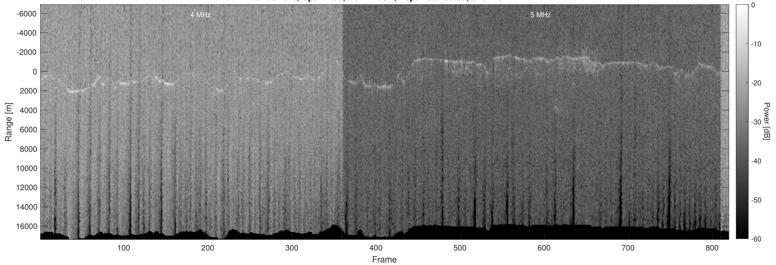
Orbit 4618, Optimized, No Window, Depth-Corrected, Channel 2
