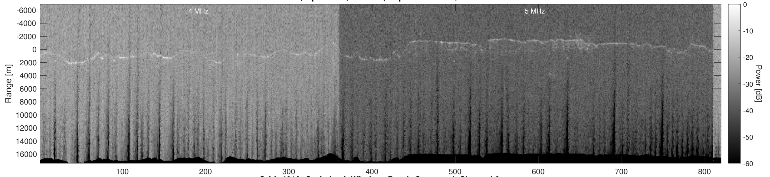
Orbit 4618, Optimized, Window, Depth-Corrected, Channel 2
