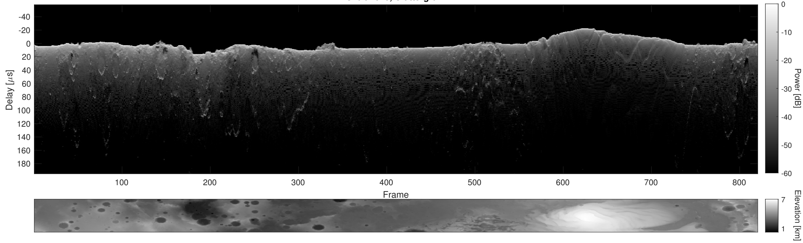
Orbit 4620, Cluttergram
