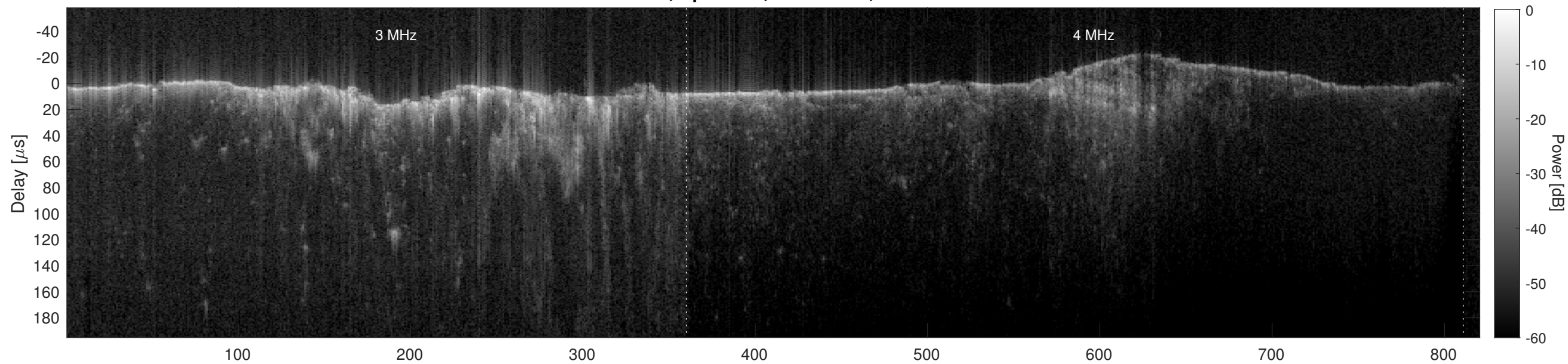
Orbit 4620, Cluttergram
