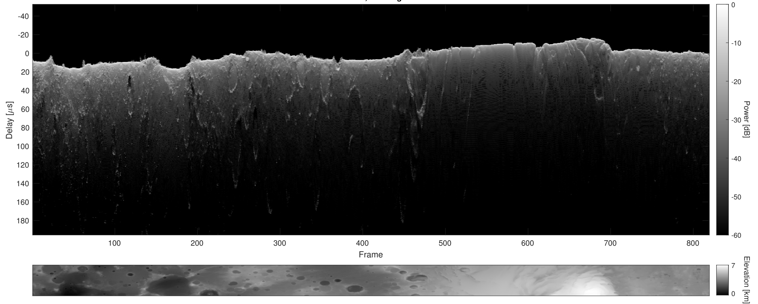
Orbit 4621, Cluttergram
