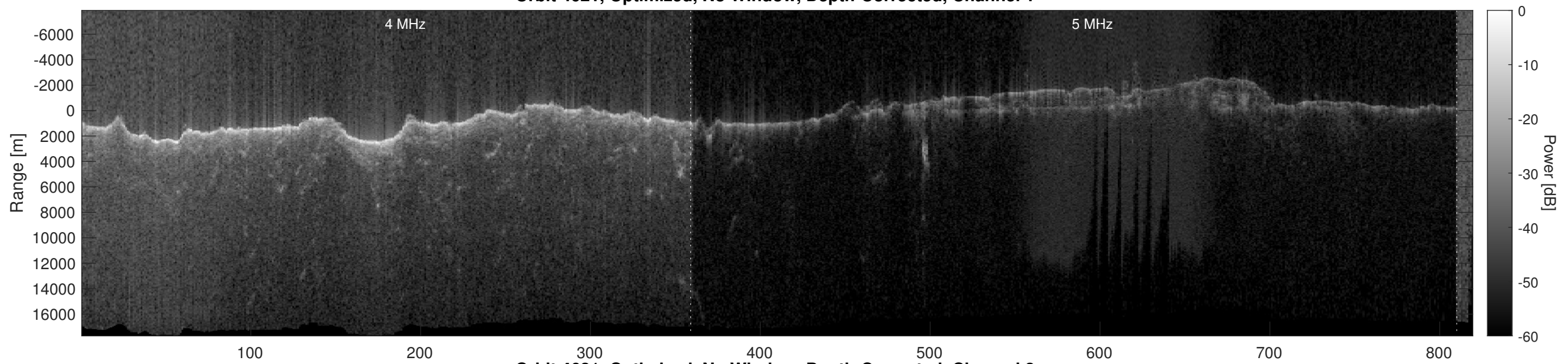
Orbit 4621, Optimized, No Window, Depth-Corrected, Channel 2
