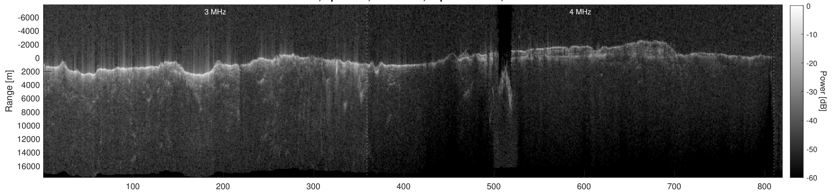
Orbit 4621, Depth-Corrected Cluttergram
