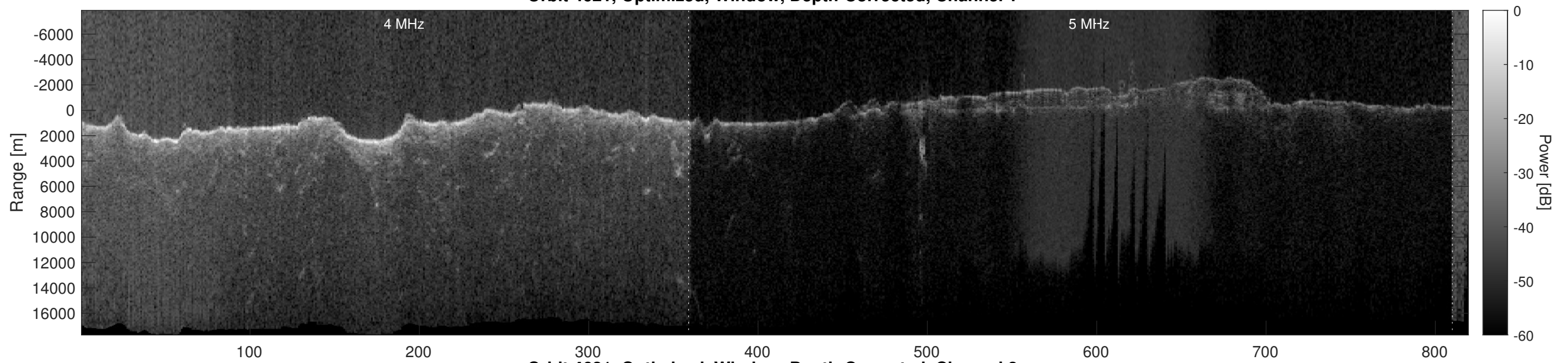
Orbit 4621, Optimized, Window, Depth-Corrected, Channel 2
