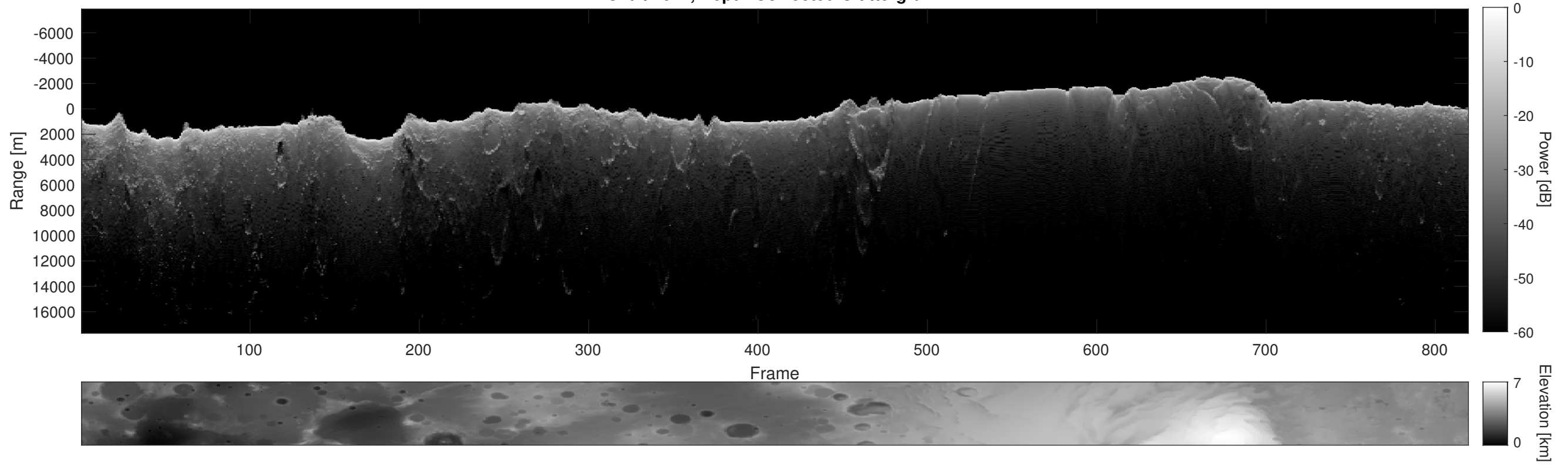
Orbit 4621, Depth-Corrected Cluttergram
