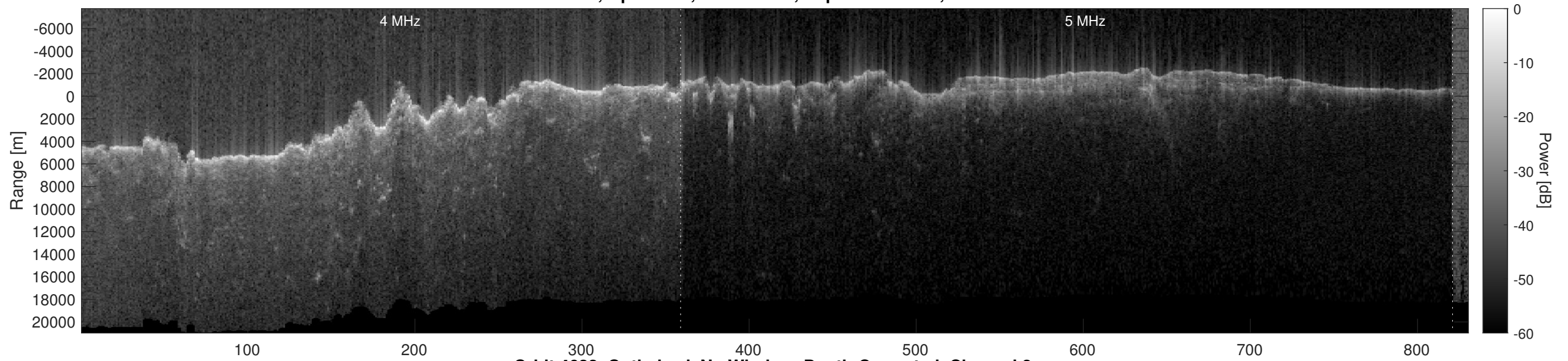
Orbit 4622, Optimized, No Window, Depth-Corrected, Channel 2
