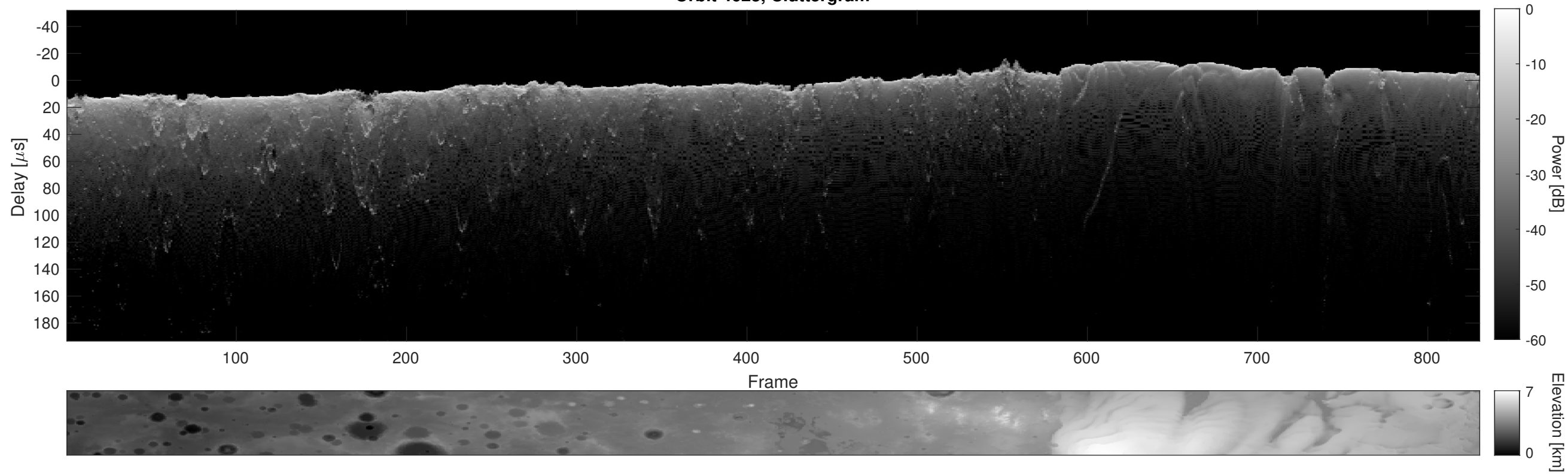
Orbit 4623, Cluttergram
