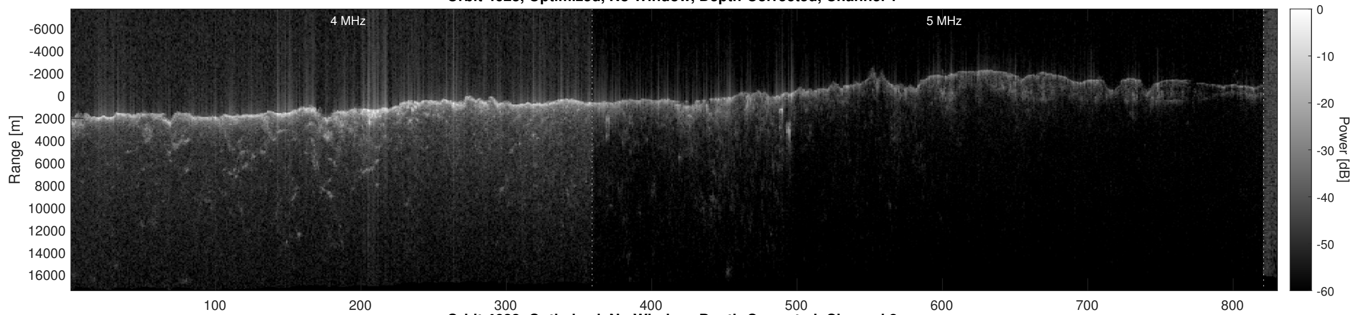
Orbit 4623, Optimized, No Window, Depth-Corrected, Channel 2
