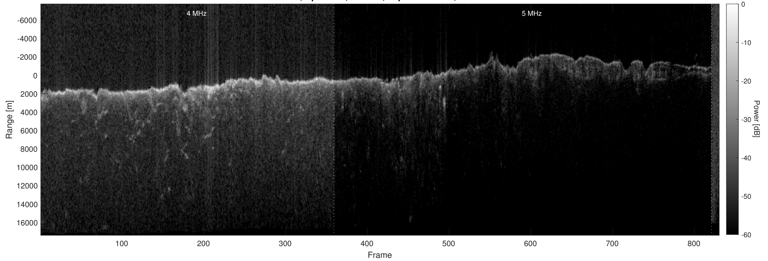
Orbit 4623, Optimized, Window, Depth-Corrected, Channel 2
