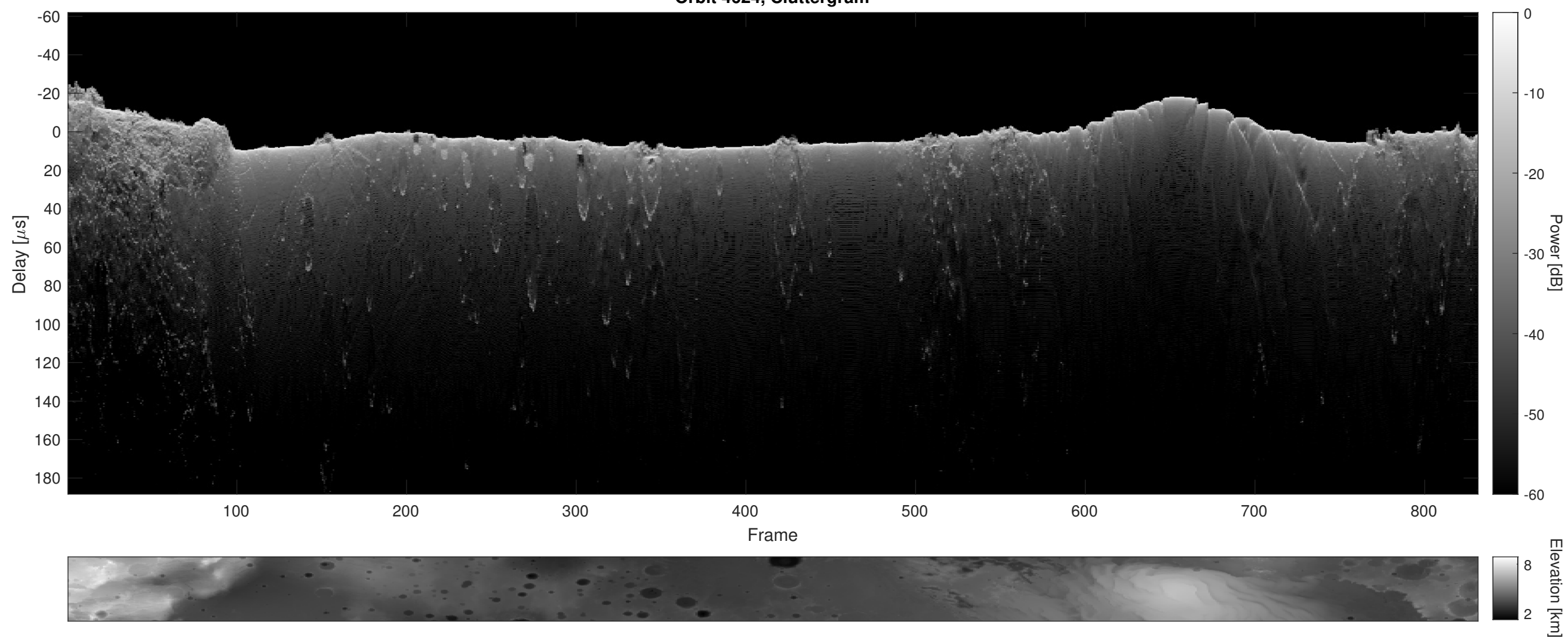
Orbit 4624, Cluttergram
