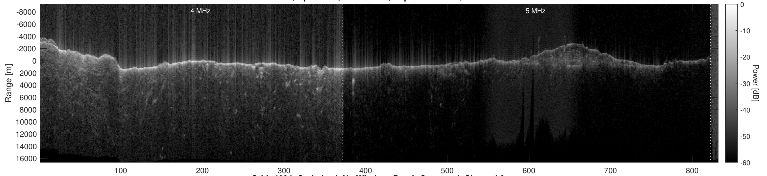
Orbit 4624, Optimized, No Window, Depth-Corrected, Channel 2
