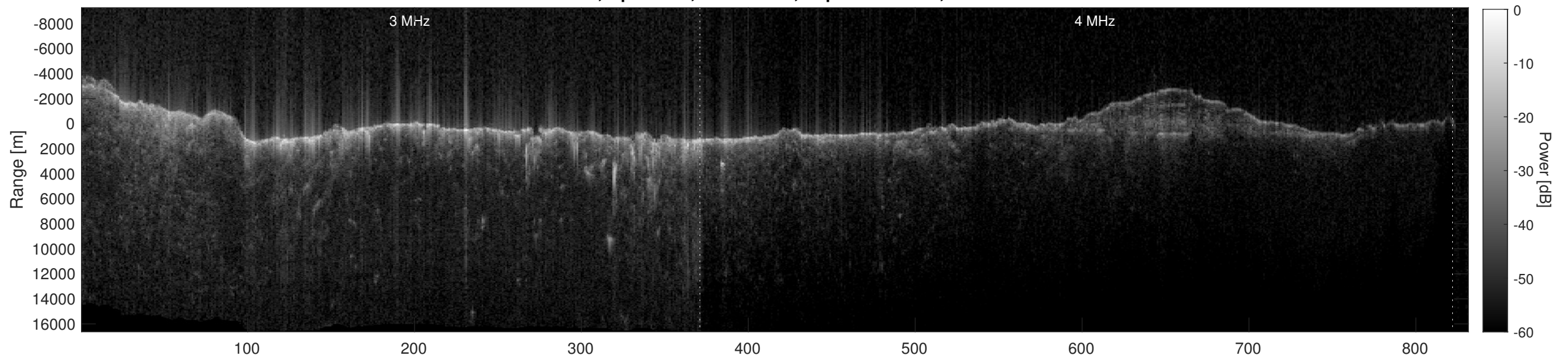
Orbit 4624, Depth-Corrected Cluttergram
