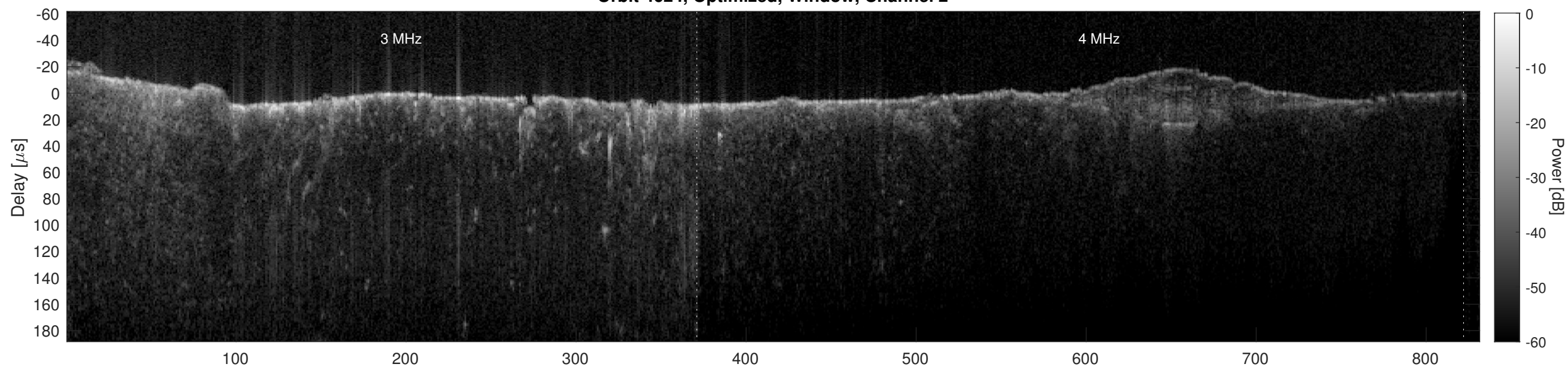
Orbit 4624, Cluttergram
