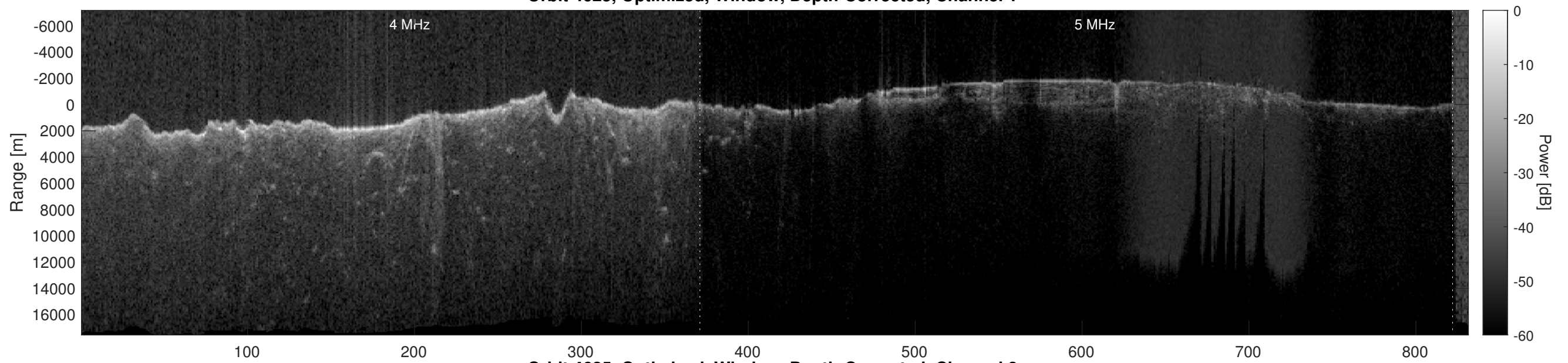
Orbit 4625, Optimized, Window, Depth-Corrected, Channel 2
