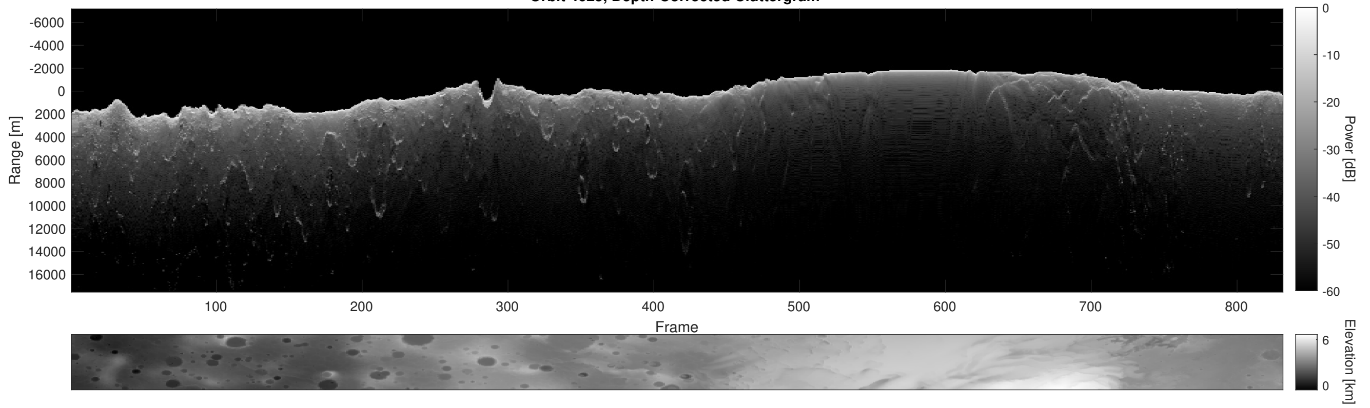
Orbit 4625, Depth-Corrected Cluttergram
