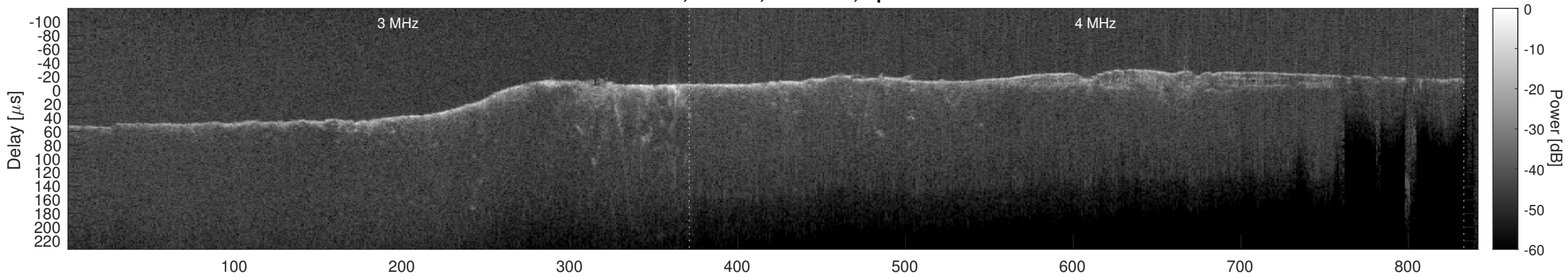
Orbit 4626, Cluttergram
