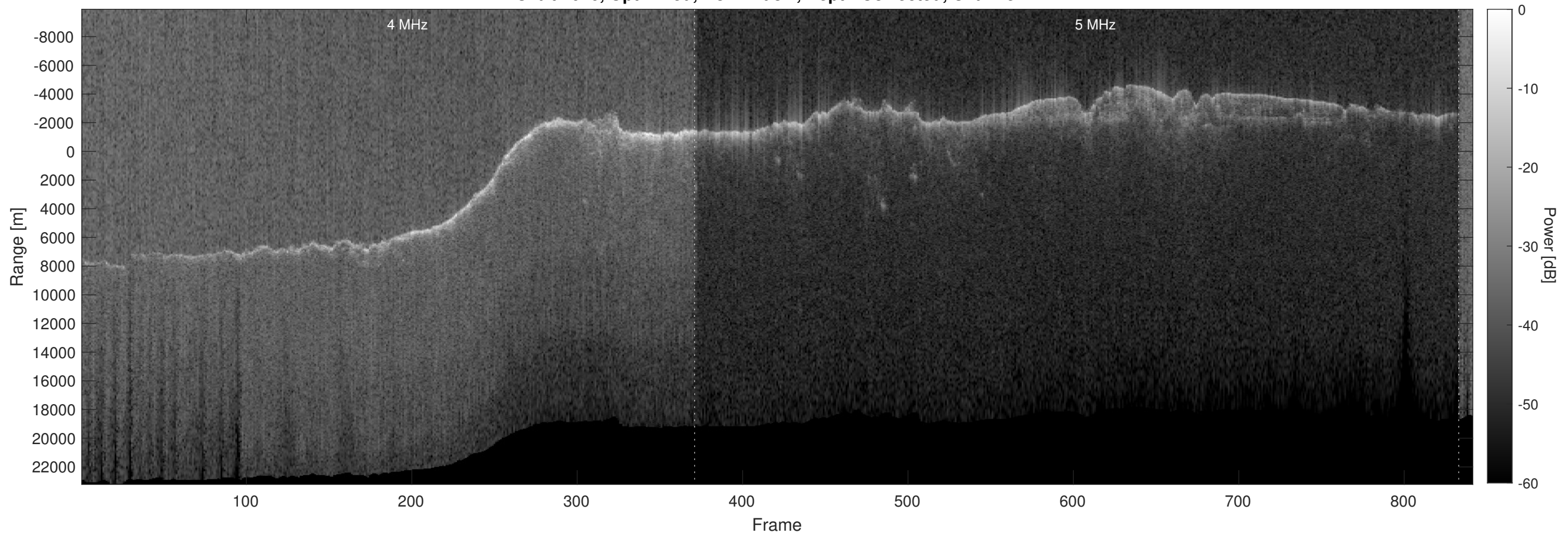
Orbit 4626, Optimized, No Window, Depth-Corrected, Channel 2
