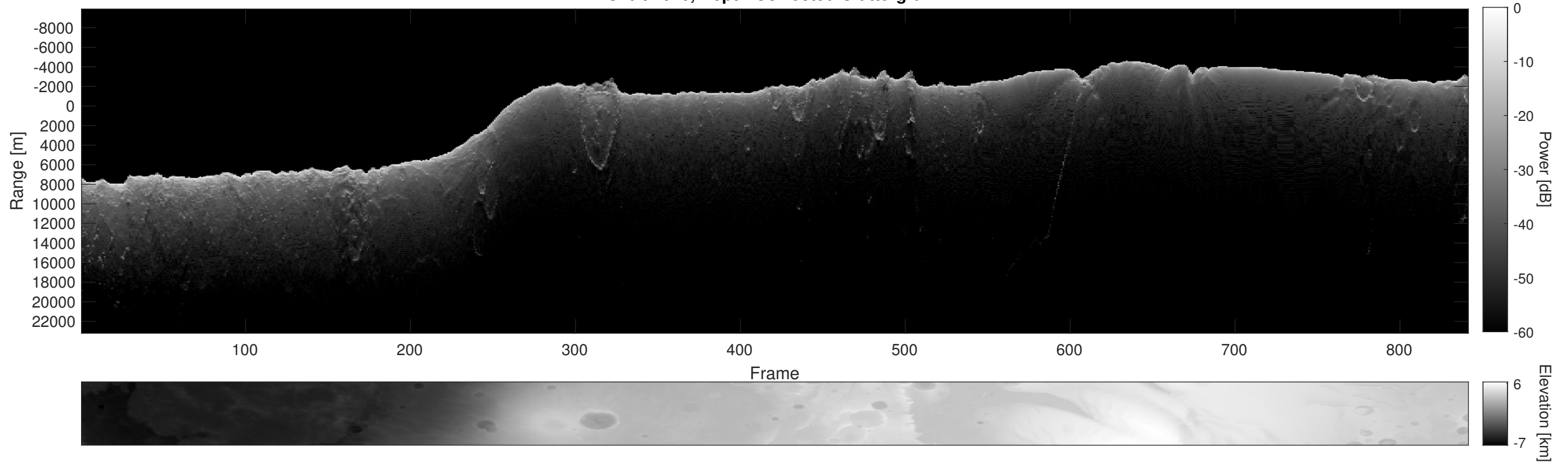
Orbit 4626, Depth-Corrected Cluttergram
