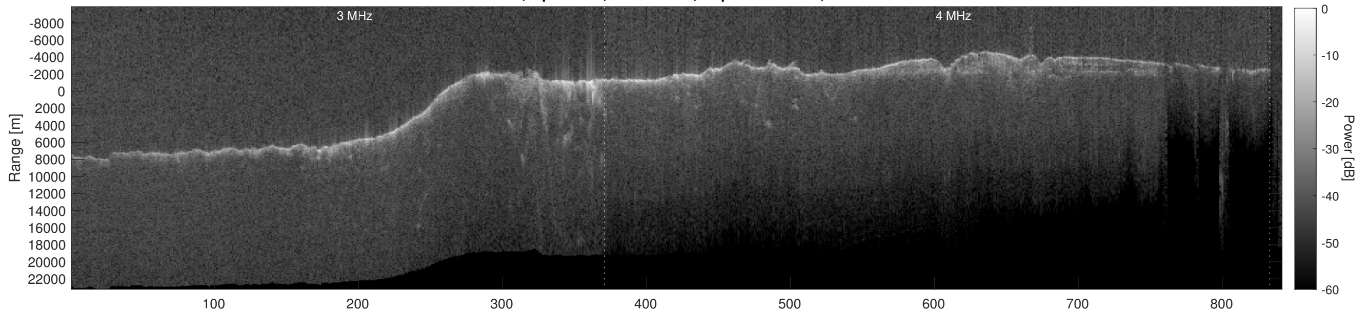
Orbit 4626, Depth-Corrected Cluttergram
