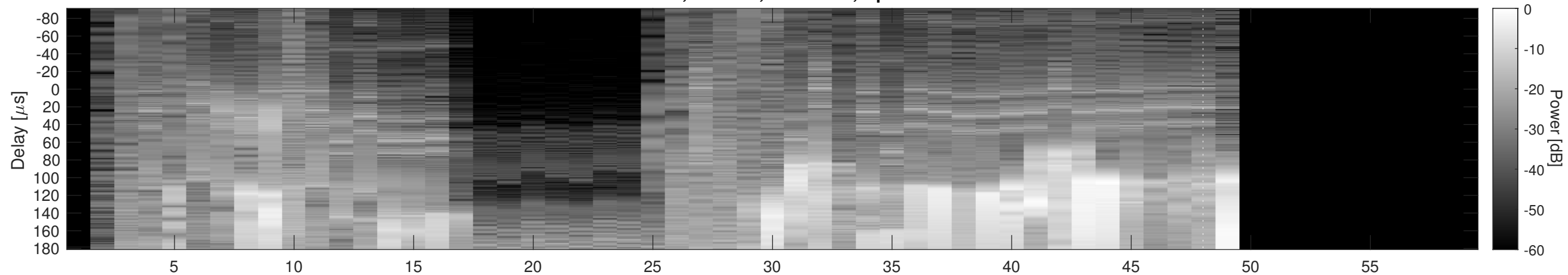
Orbit 4628, Cluttergram
