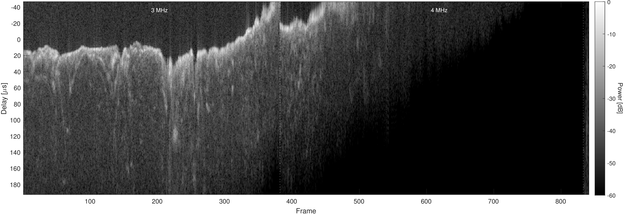
Orbit 4629, Chapman, Window, Channel 2
