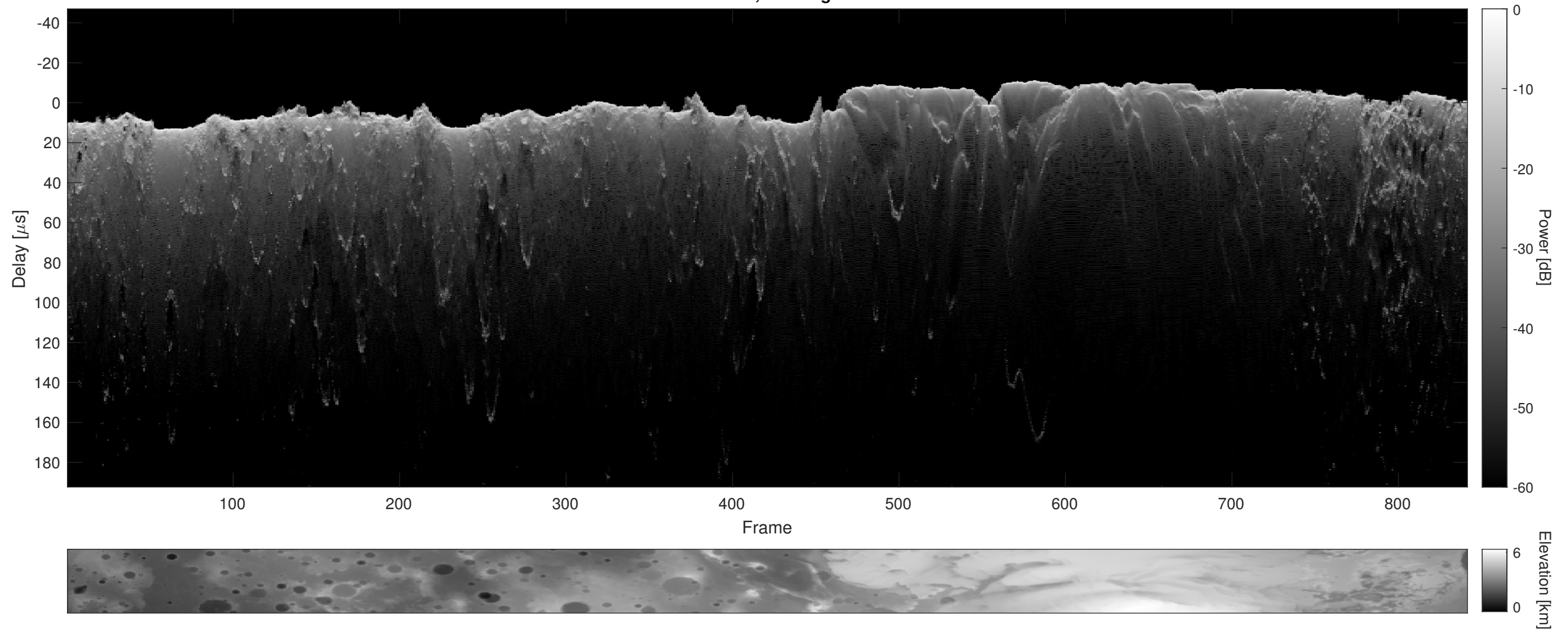
Orbit 4629, Cluttergram
