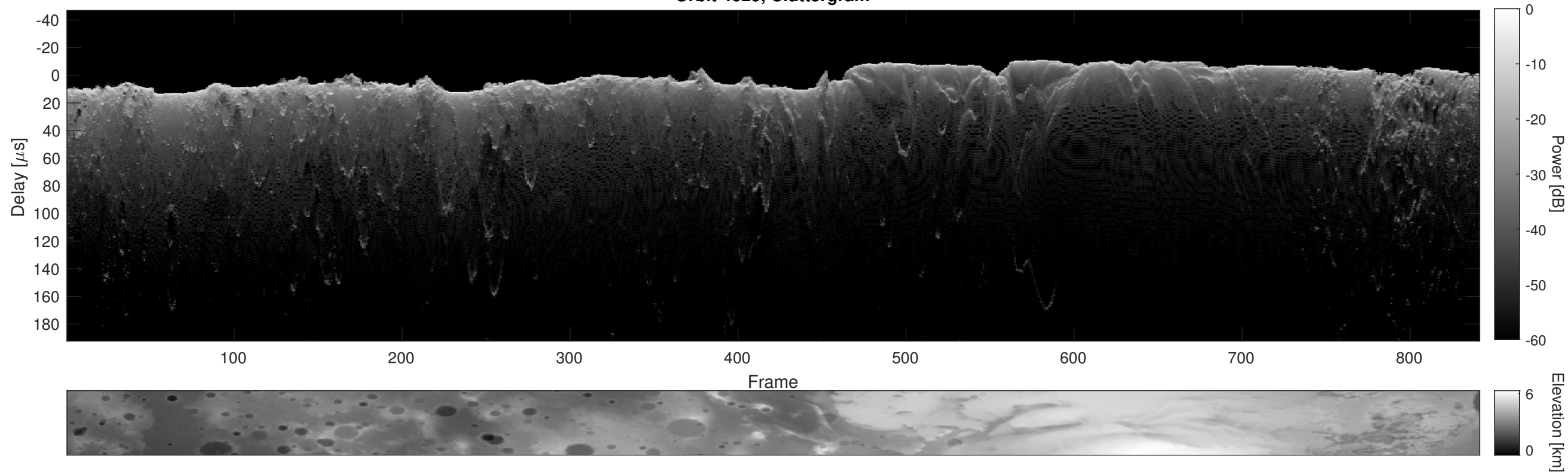
Orbit 4629, Cluttergram
