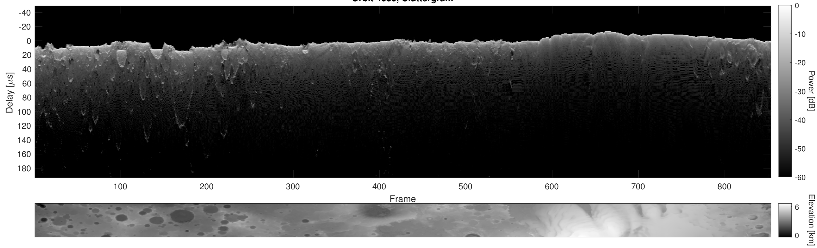
Orbit 4630, Cluttergram
