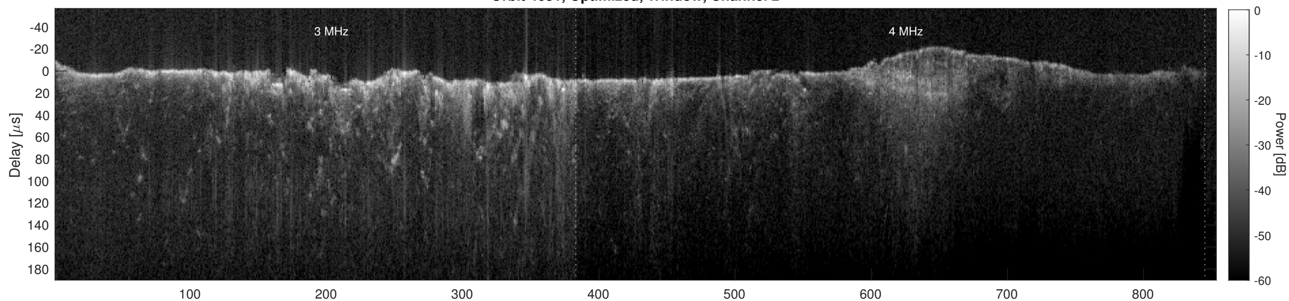
Orbit 4631, Cluttergram
