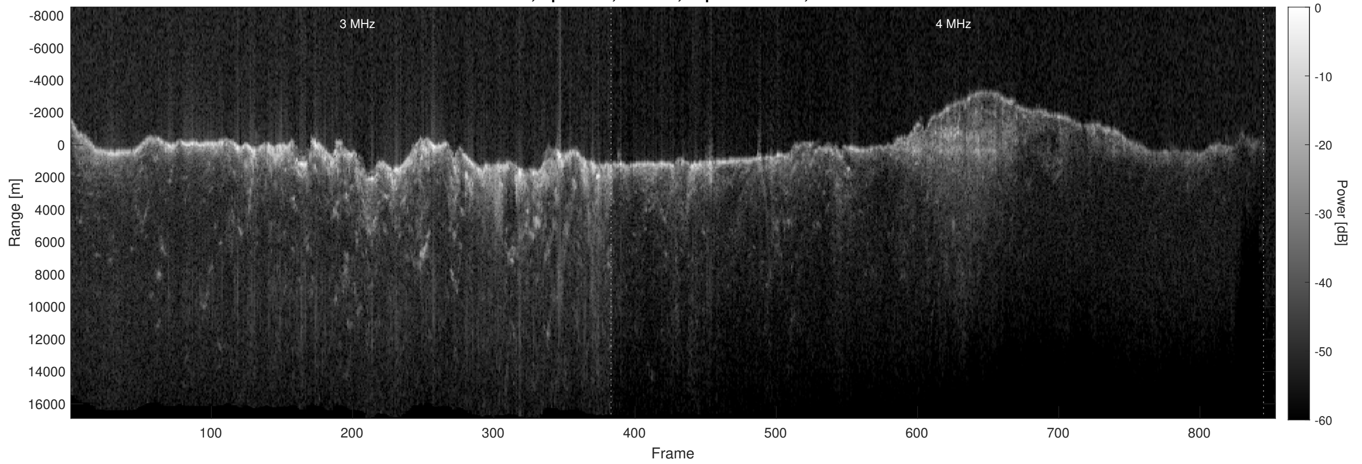
Orbit 4631, Optimized, Window, Depth-Corrected, Channel 2
