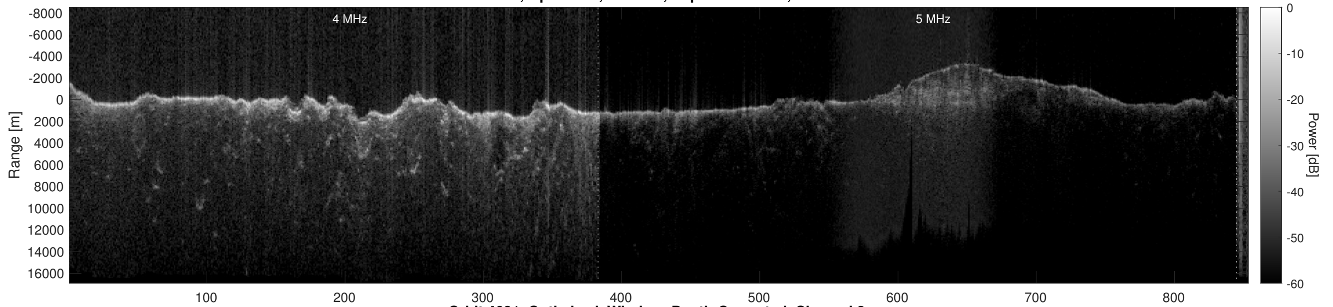
Orbit 4631, Optimized, Window, Depth-Corrected, Channel 2
