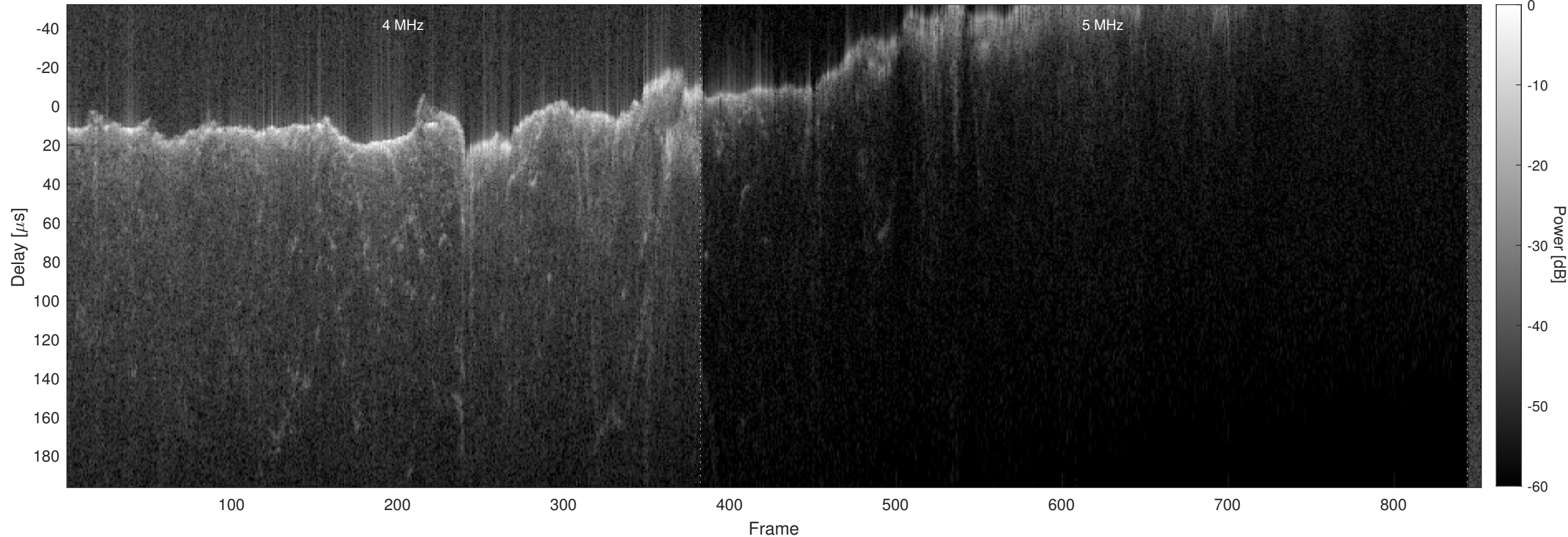
Orbit 4632, Chapman, No Window, Channel 2
