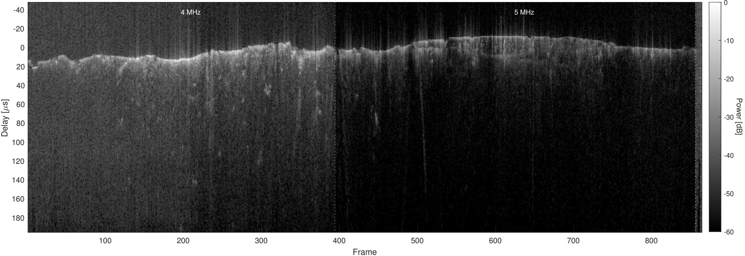
Orbit 4636, Optimized, No Window, Channel 2
