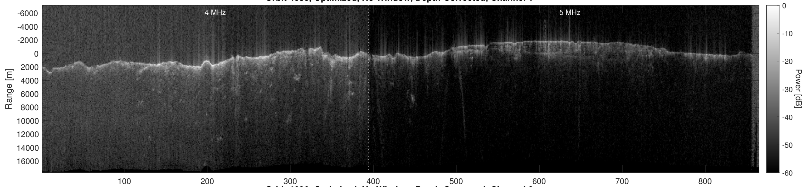
Orbit 4636, Optimized, No Window, Depth-Corrected, Channel 2
