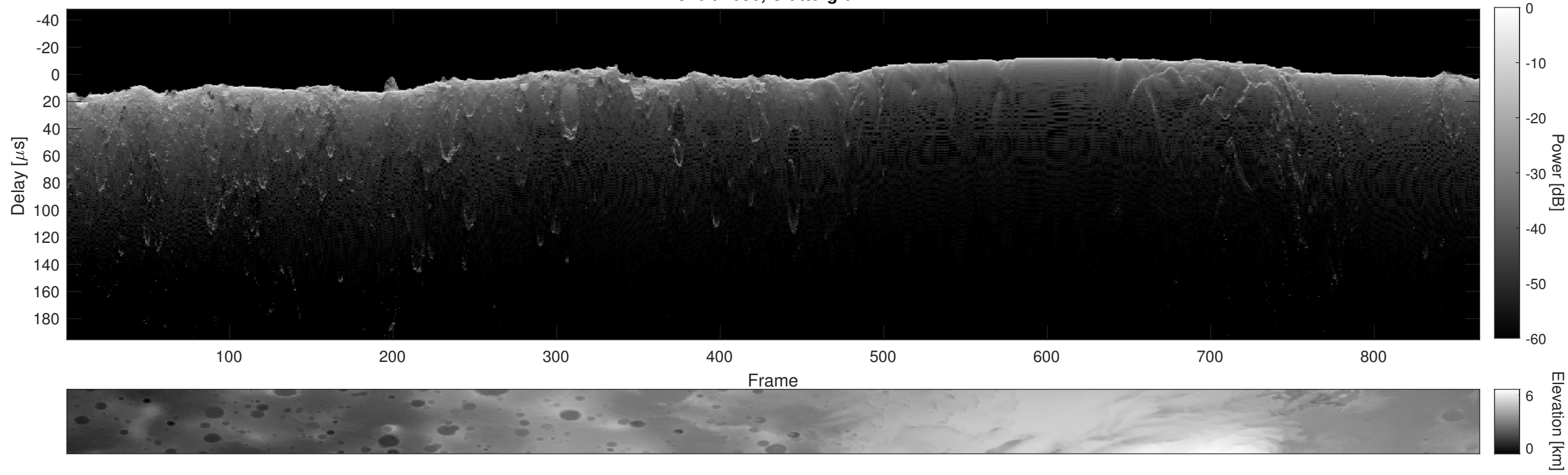
Orbit 4636, Cluttergram
