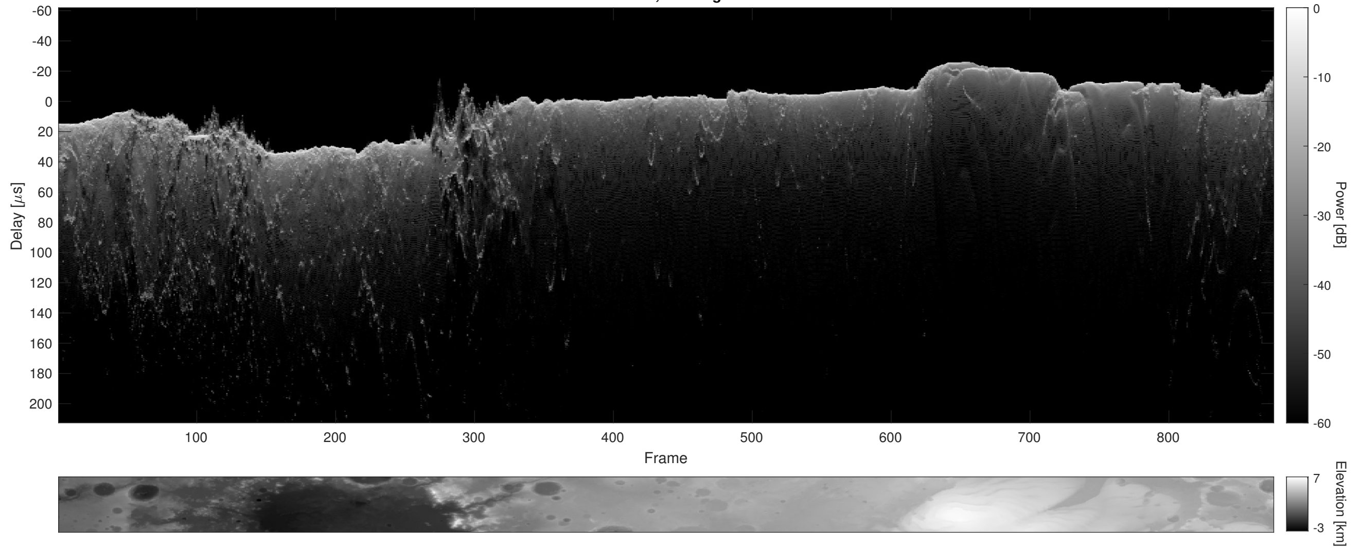
Orbit 4638, Cluttergram
