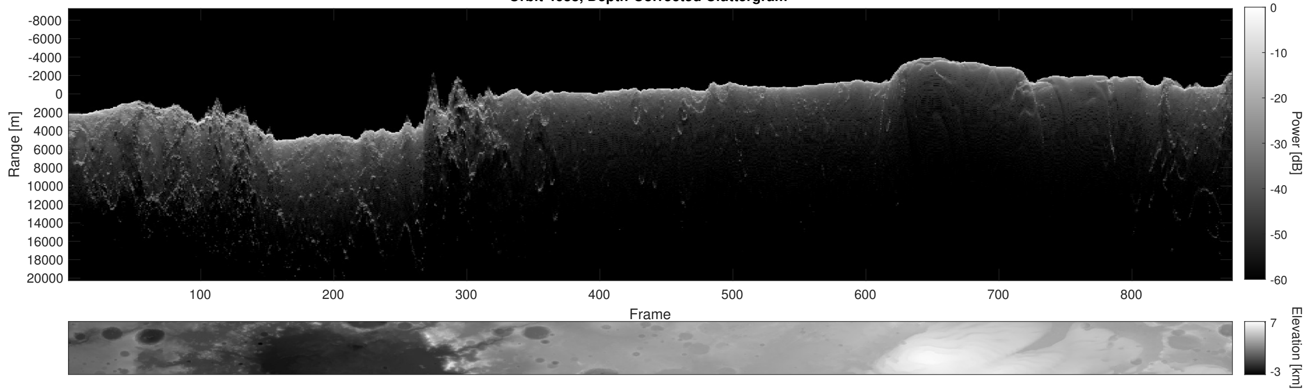
Orbit 4638, Depth-Corrected Cluttergram
