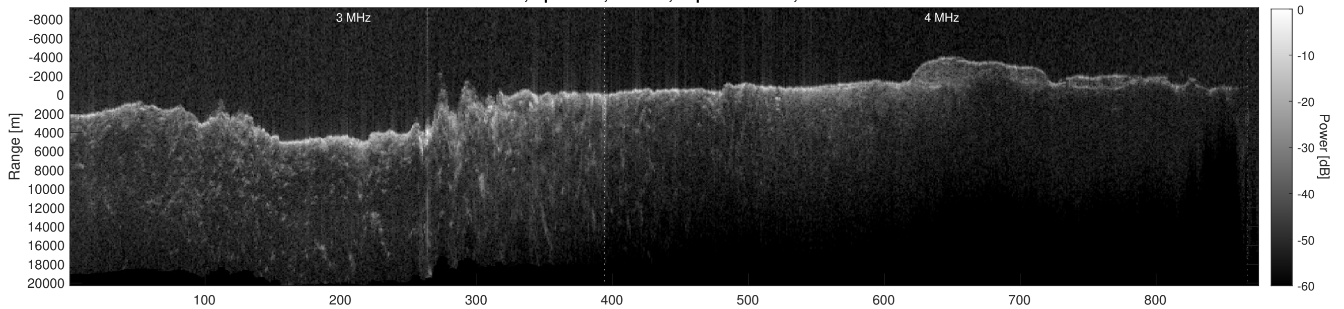
Orbit 4638, Depth-Corrected Cluttergram
