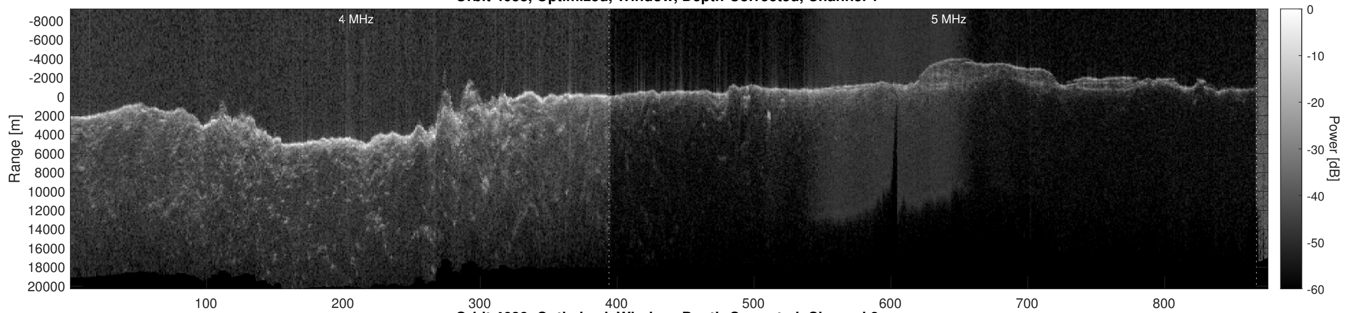
Orbit 4638, Optimized, Window, Depth-Corrected, Channel 2
