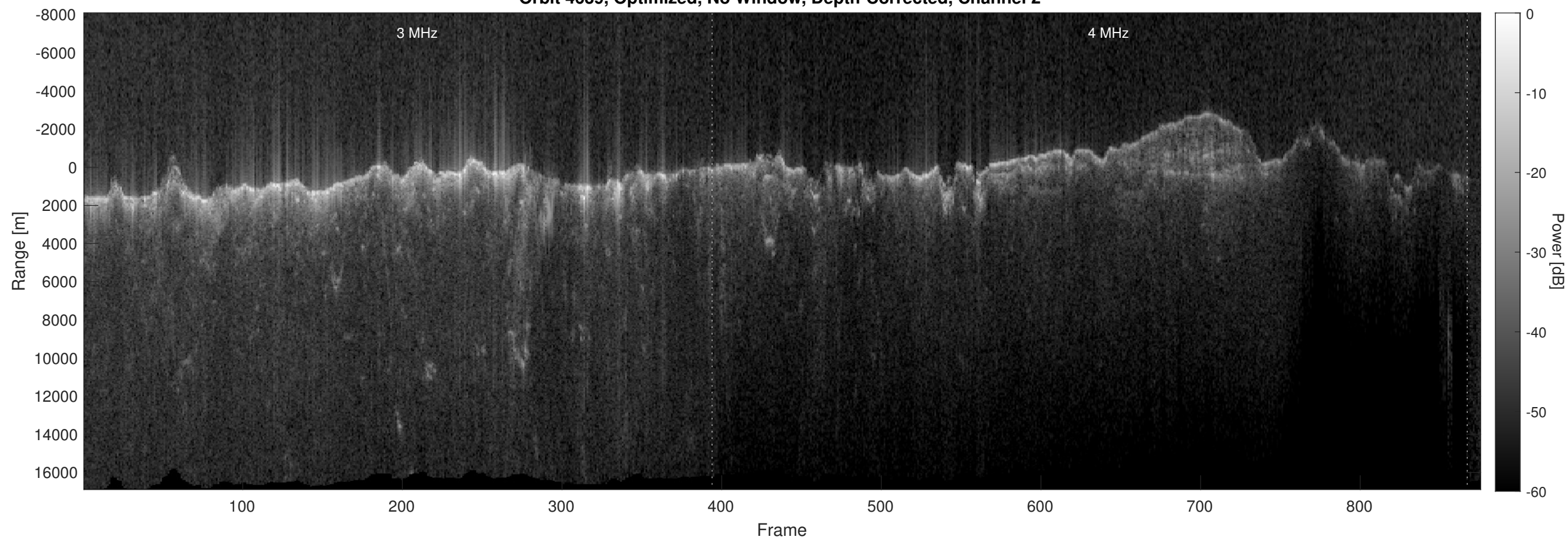
Orbit 4639, Optimized, No Window, Depth-Corrected, Channel 2
