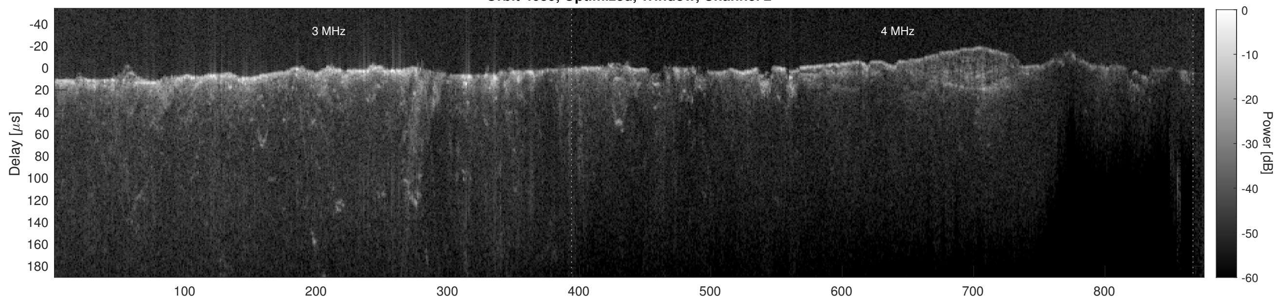
Orbit 4639, Cluttergram
