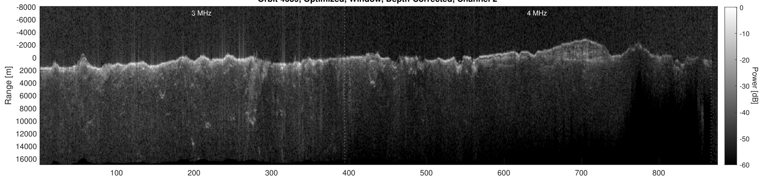
Orbit 4639, Depth-Corrected Cluttergram
