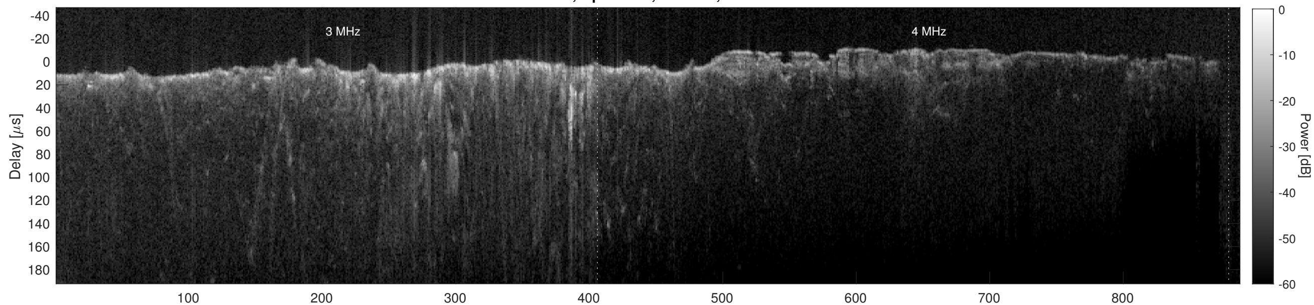
Orbit 4640, Cluttergram
