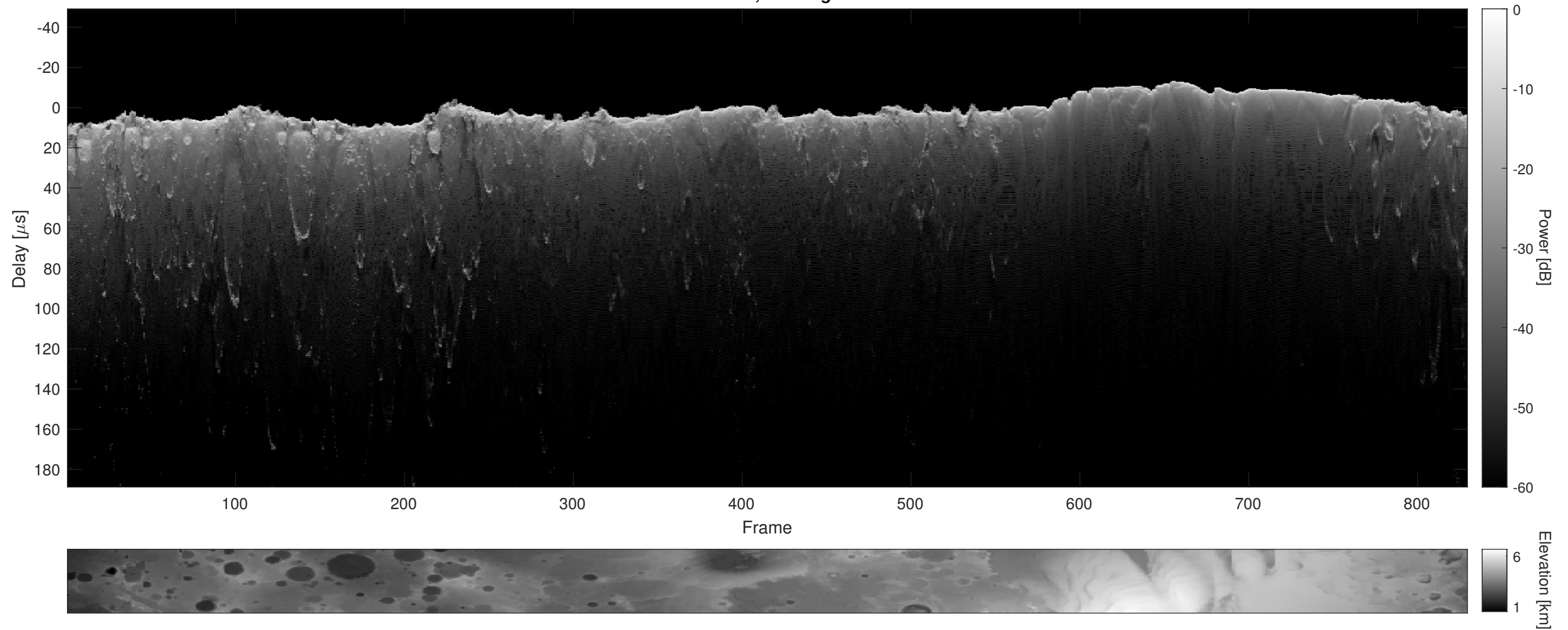
Orbit 4641, Cluttergram
