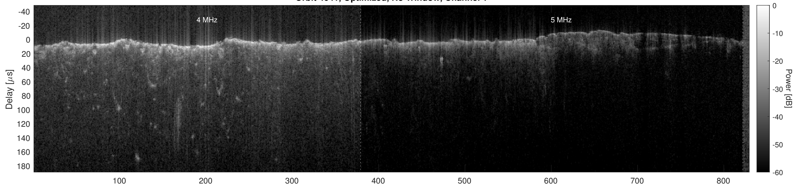
Orbit 4641, Optimized, No Window, Channel 2
