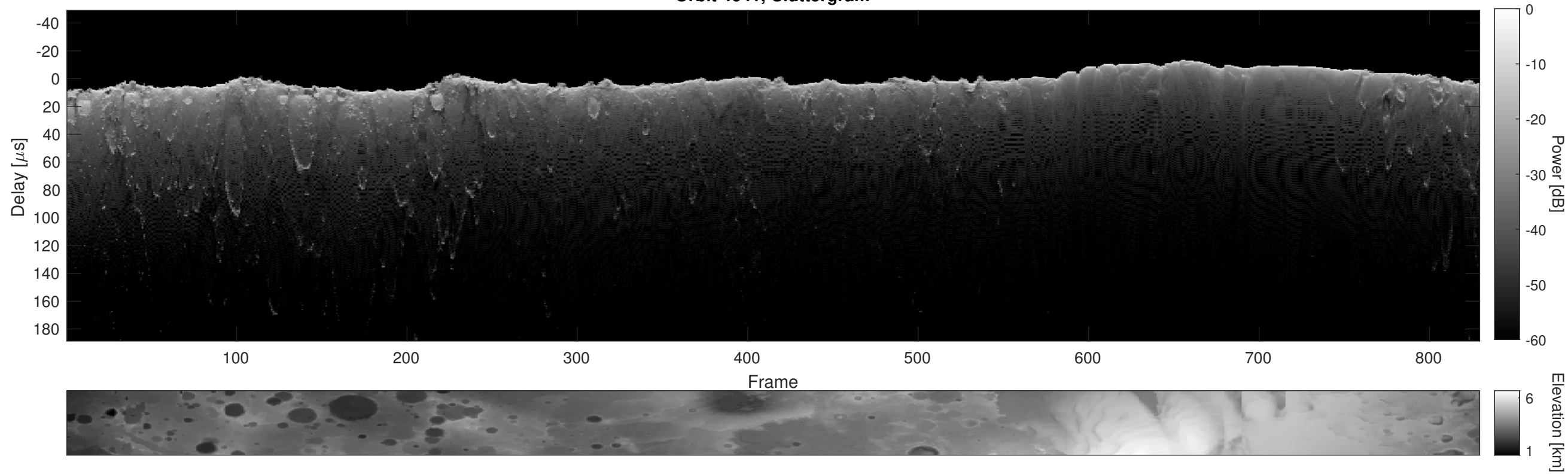
Orbit 4641, Cluttergram
