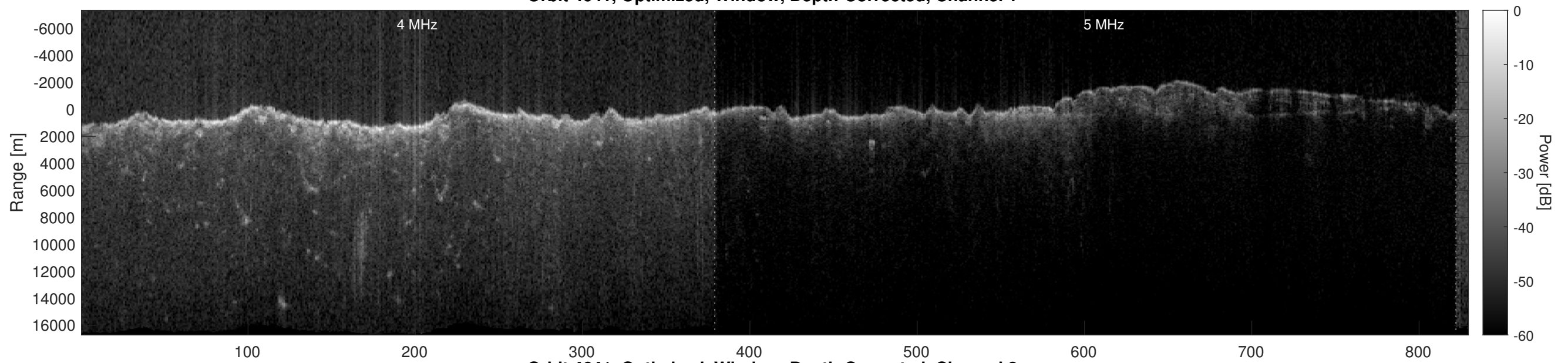
Orbit 4641, Optimized, Window, Depth-Corrected, Channel 2
