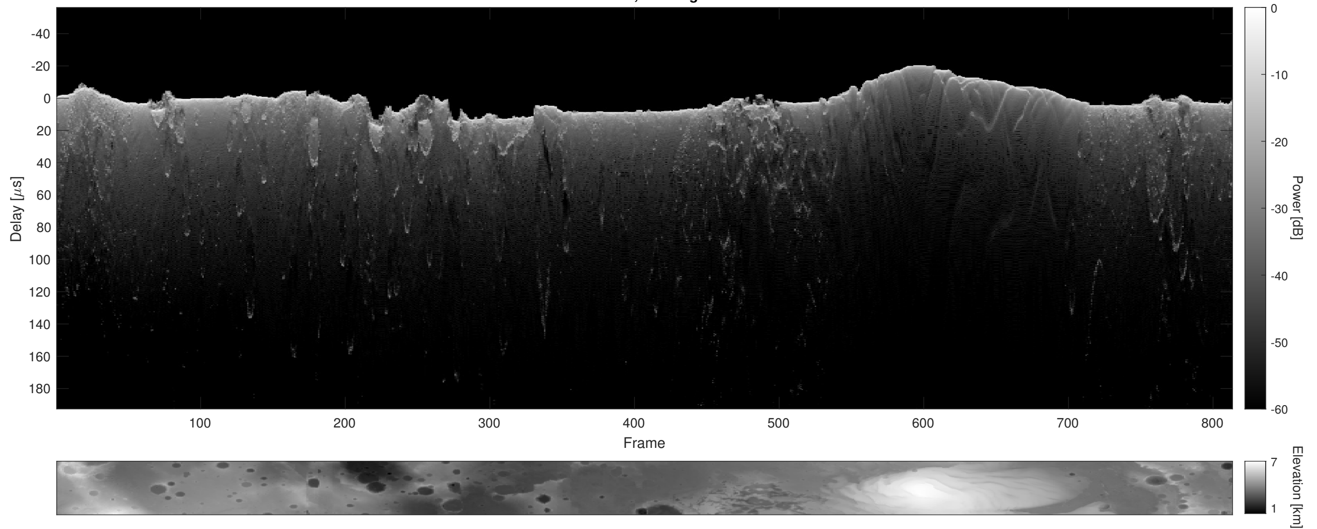
Orbit 4642, Cluttergram
