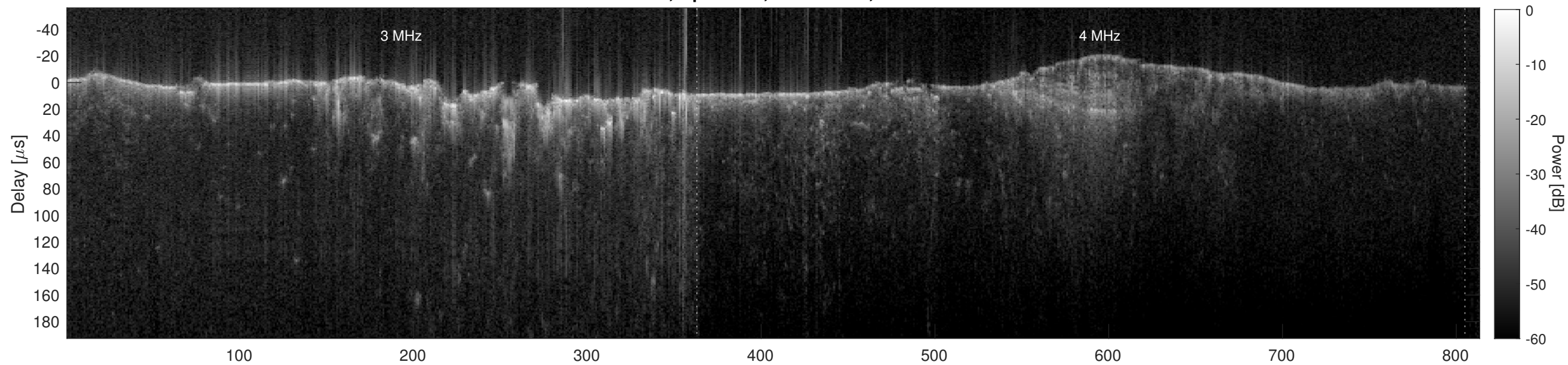
Orbit 4642, Cluttergram
