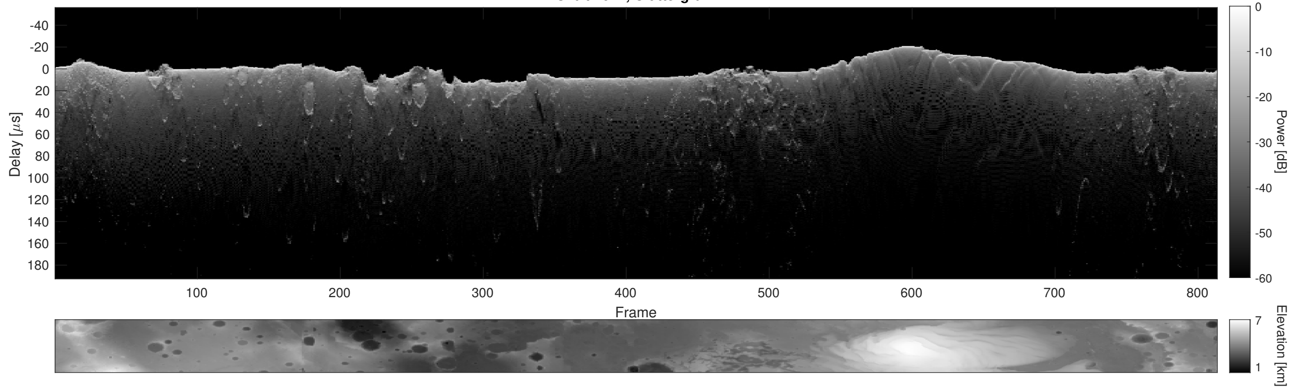
Orbit 4642, Cluttergram
