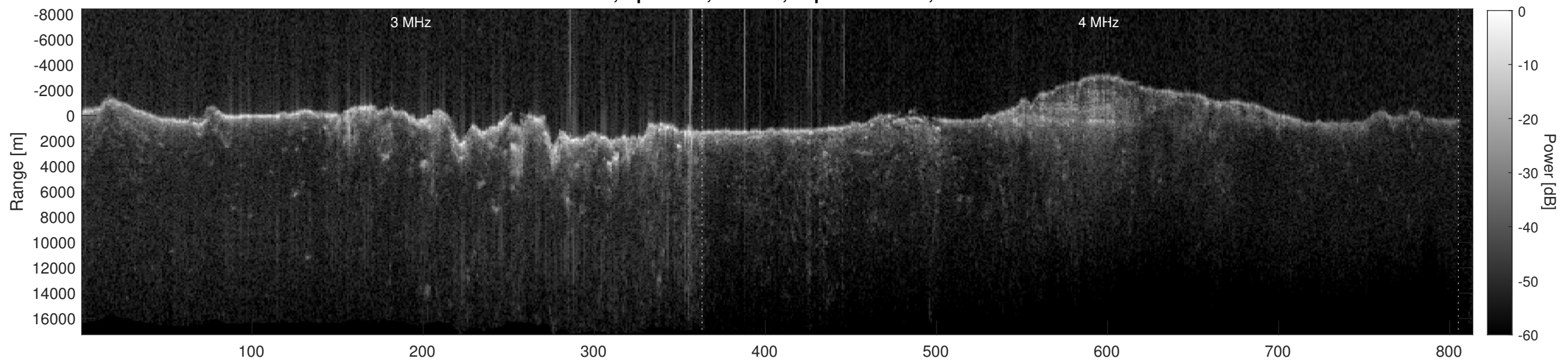
Orbit 4642, Depth-Corrected Cluttergram
