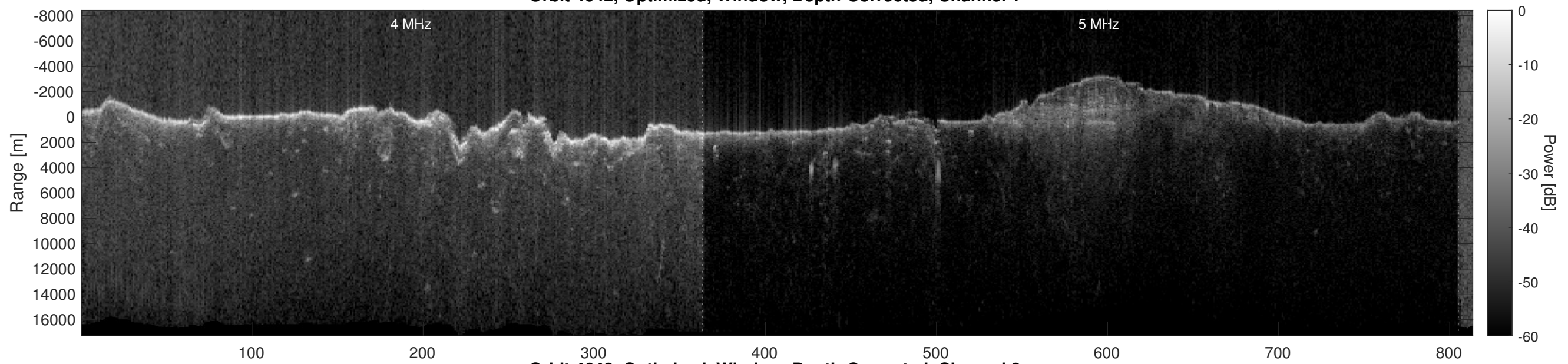
Orbit 4642, Optimized, Window, Depth-Corrected, Channel 2
