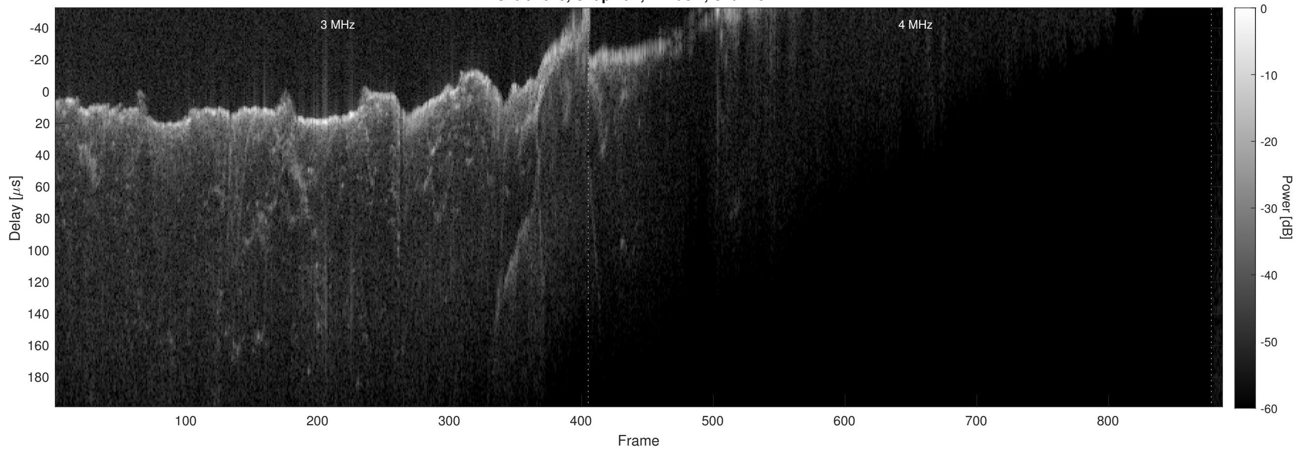
Orbit 4643, Chapman, Window, Channel 2
