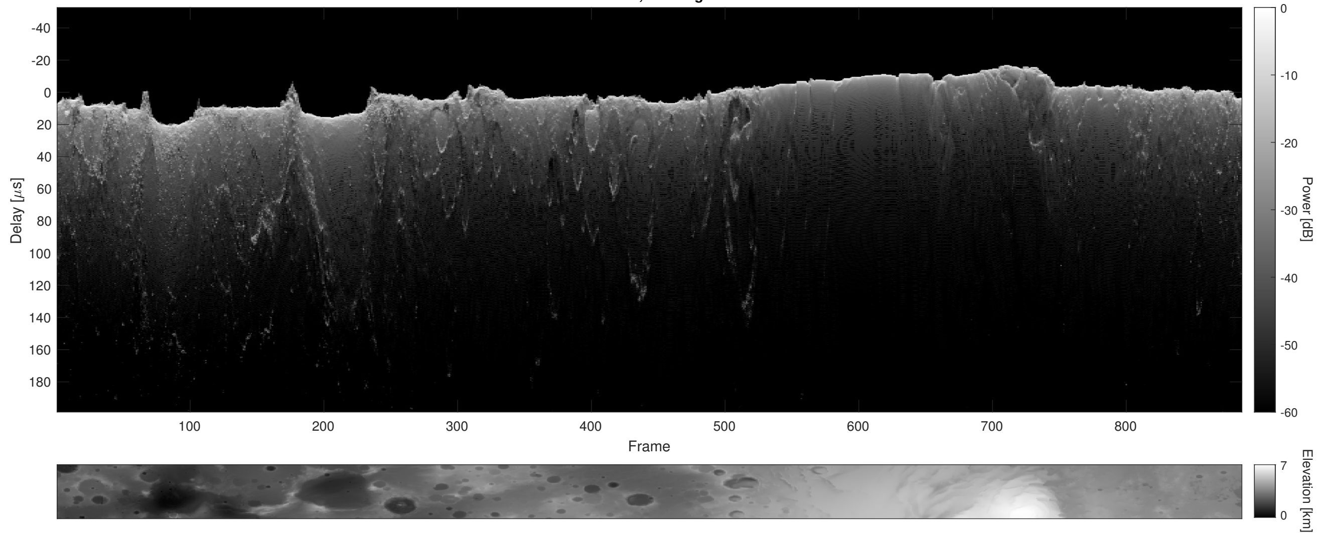
Orbit 4643, Cluttergram
