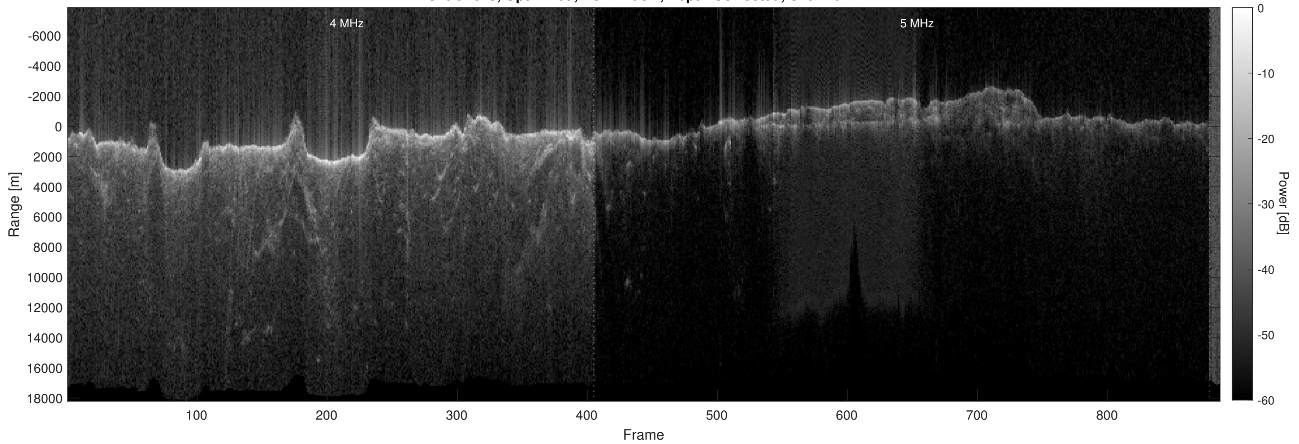
Orbit 4643, Optimized, No Window, Depth-Corrected, Channel 2
