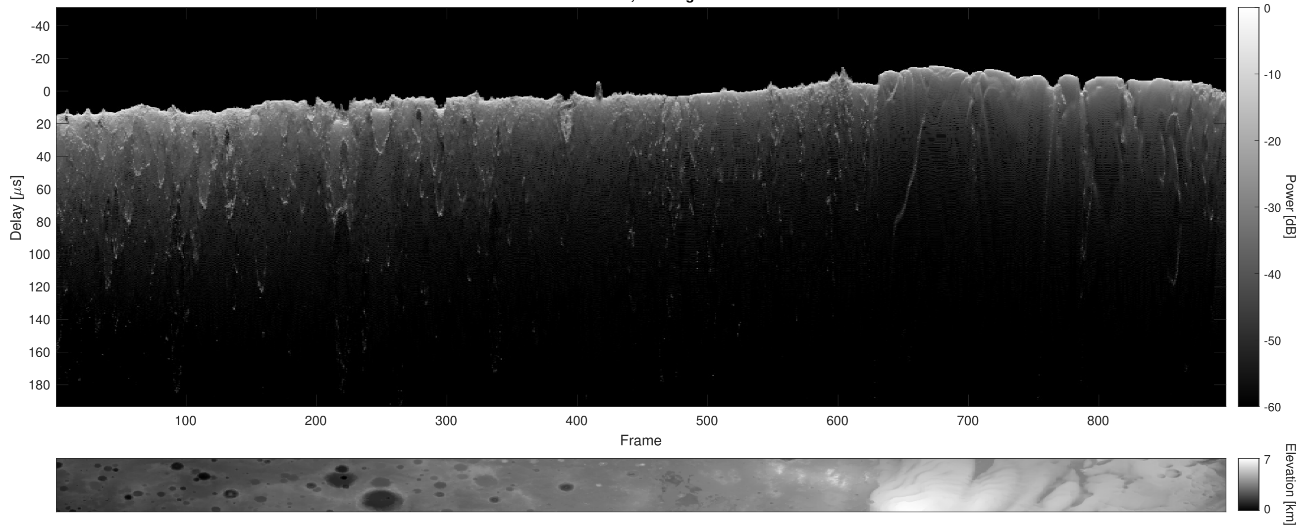
Orbit 4645, Cluttergram
