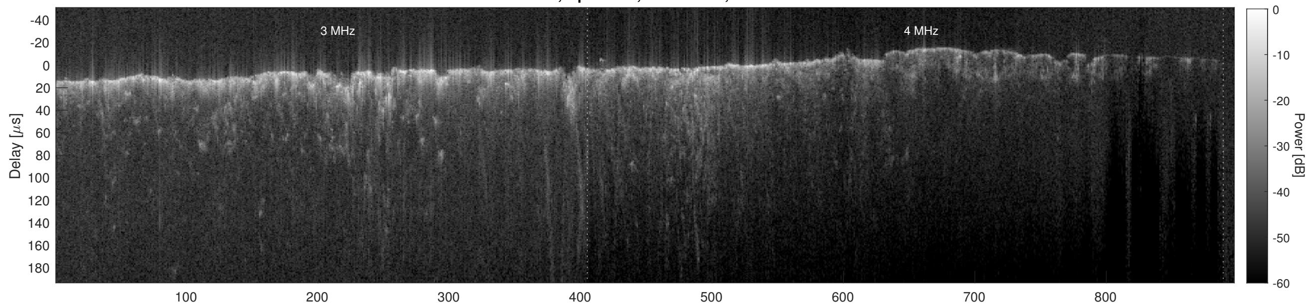
Orbit 4645, Cluttergram
