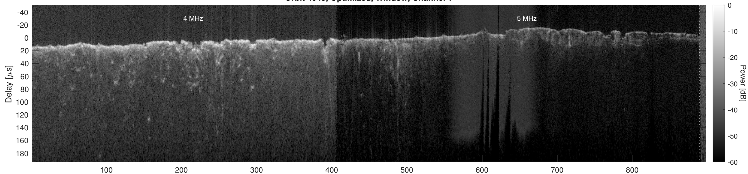
Orbit 4645, Optimized, Window, Channel 2
