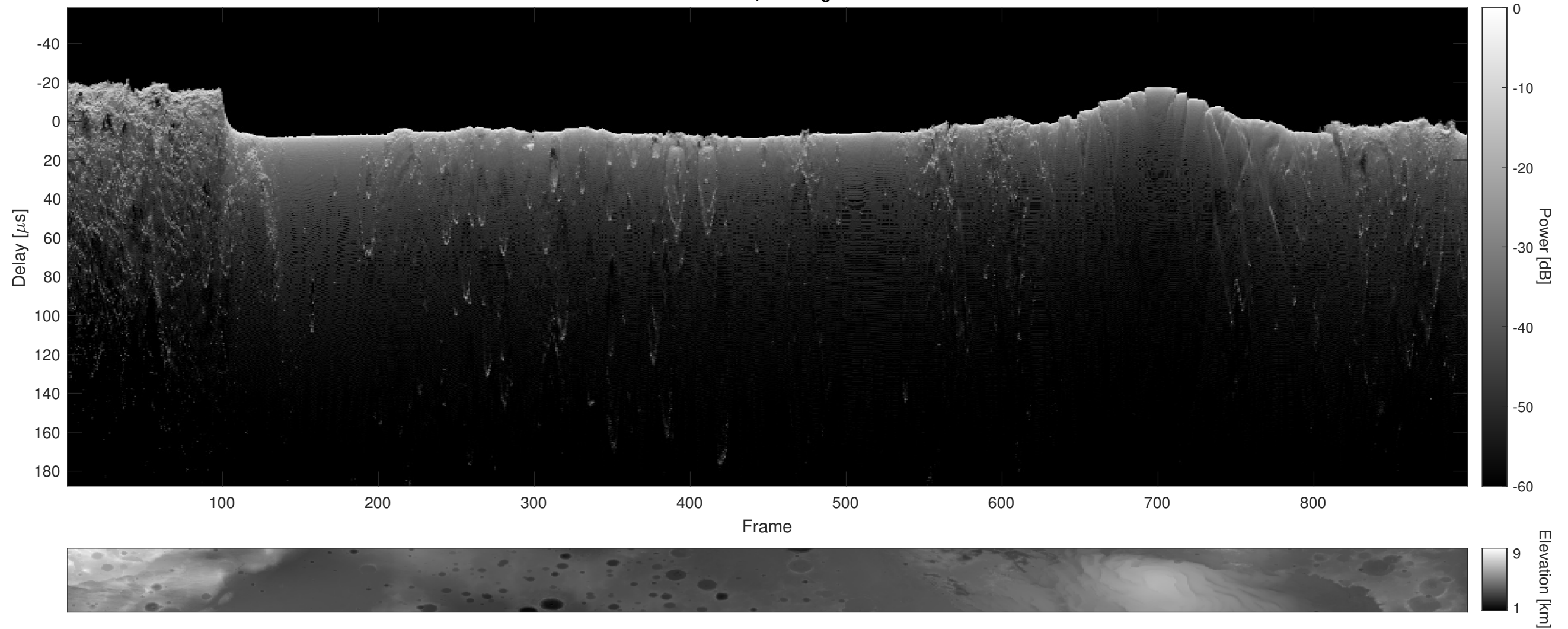
Orbit 4646, Cluttergram
