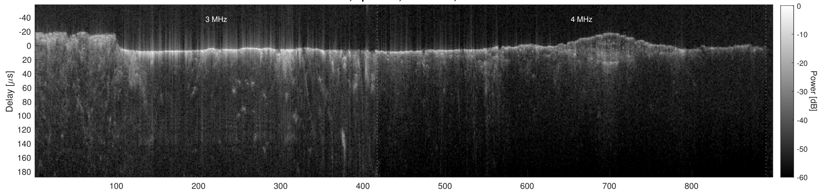
Orbit 4646, Cluttergram
